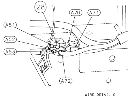
WIRE DETAILS
