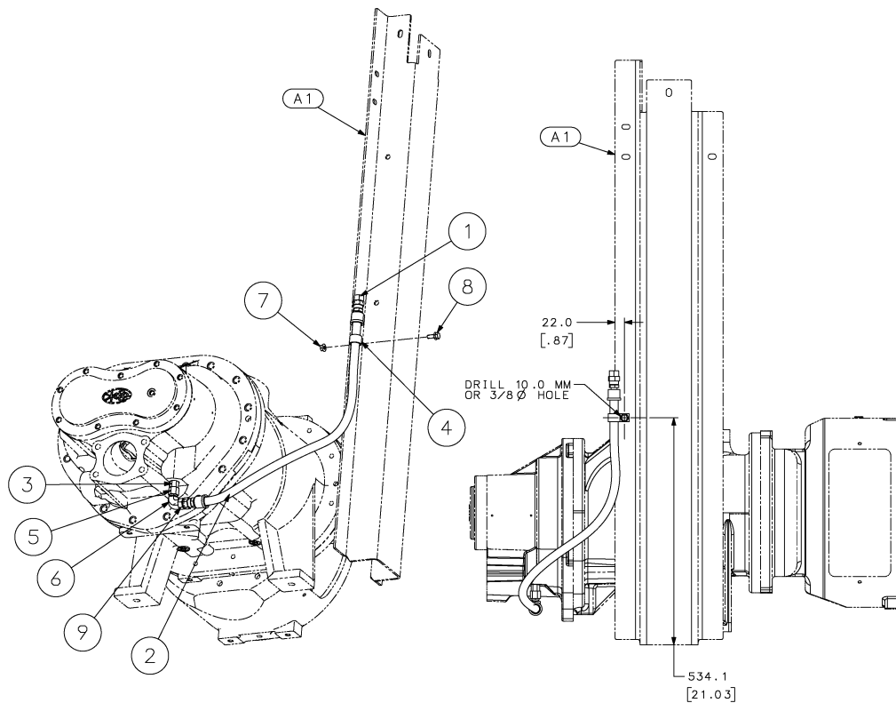
COMPRESSOR UNIT DRAIN FOR LS160 WITH 23 SERIES WITHOUT SPIRAL VALVE CONFIGURATION
